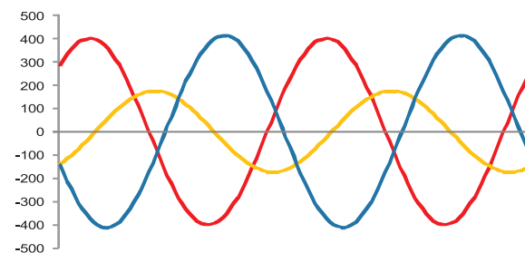
Case 2: Typical welding loads
