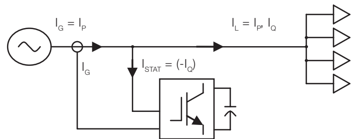
Closed loop configuration
